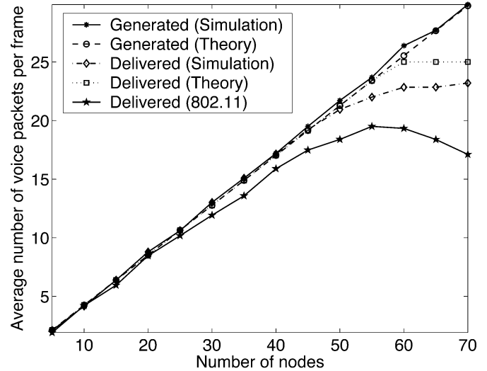
Fig. 2. Average number of voice packets per frame versus total number of nodes with active voice sources.
